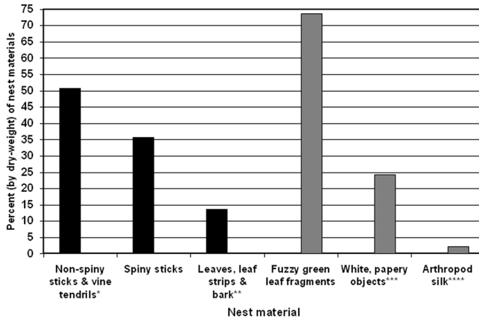
FIG. 2. Percent (by dry-weight) of various materials used in the construction of a Dusky Spinetail ( Synallaxis moesta ) nest in eastern Ecuador. The external portion of the nest (black bars) was considered separately from the internal cup lining (grey bars).
